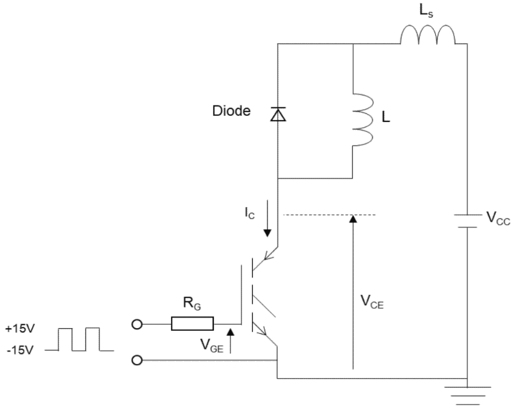
Fig. 6.1 Test Circuit
