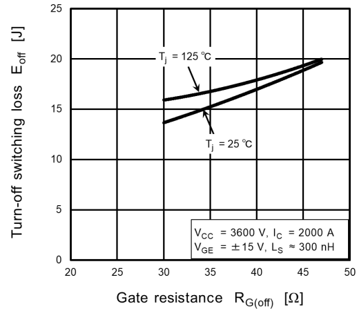
Fig. 7.8 E off - R G(off)
