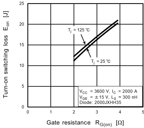
Fig. 7.7 E on - R G(on)
