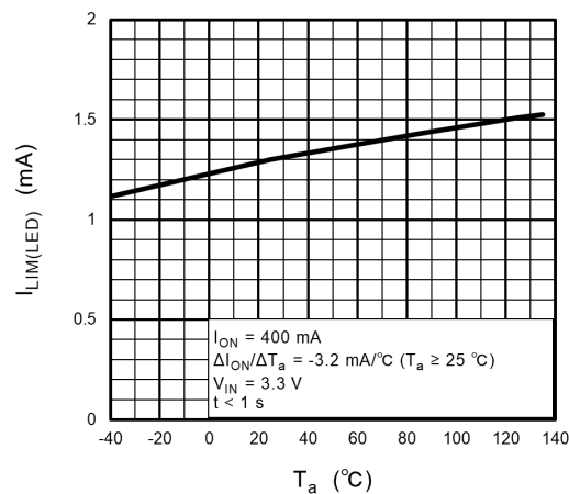
Fig. 12.7 I_{LIM(LED)} - T_a
