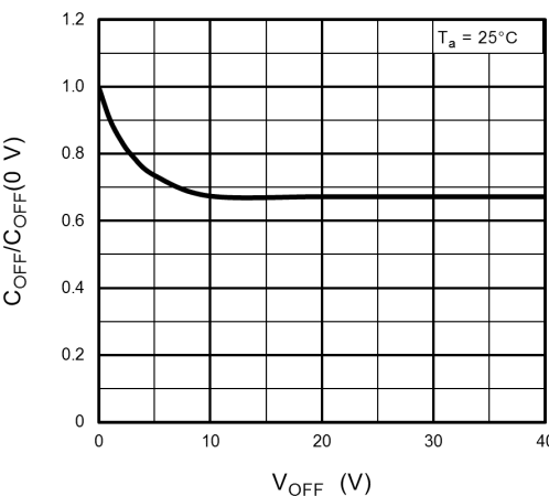
Fig. 12.12 C_{OFF}/C_{OFF}(0\text{ V}) - V_{OFF}
