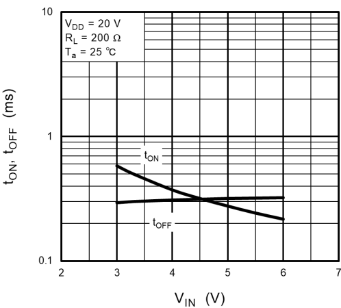
Fig. 12.8 t_{ON} , t_{OFF} - V_{IN}
