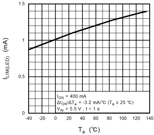
Fig. 12.7 I_{LIM(LED)} - T_a
