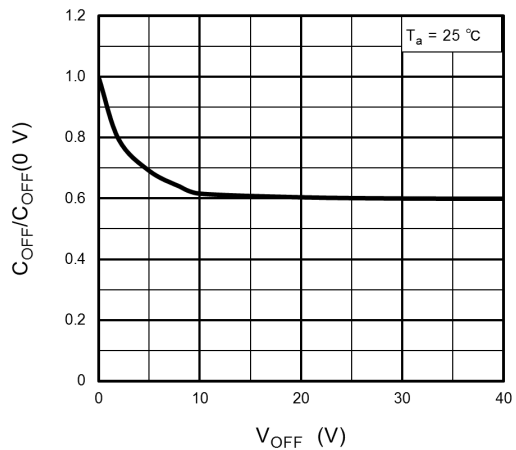
Fig. 12.12 C_{OFF}/C_{OFF(0 V)} - V_{OFF}
