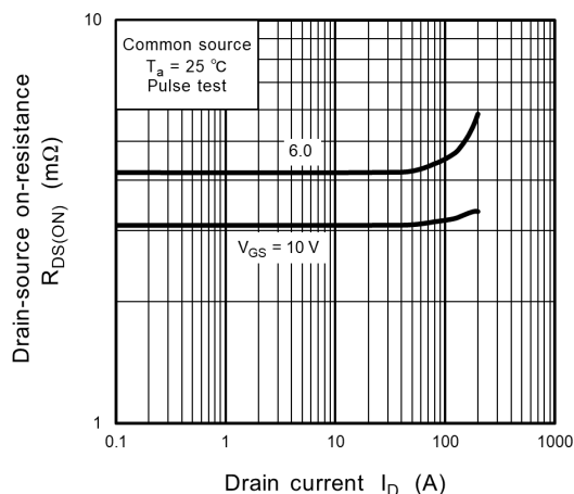
Fig. 8.8 R_{DS(ON)} - I_D
