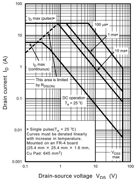
Fig. 8.9 Safe Operating Area
