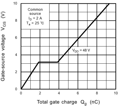
Fig. 8.8 Dynamic Input Characteristics
