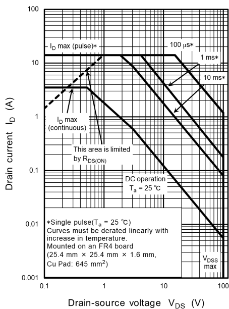
Fig. 8.10 Safe Operating Area
