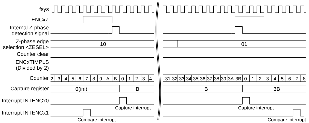
Figure 3.9 ENCxZ Input is Enabled. ( [ENxTNCR]<ZEN>=1 )
