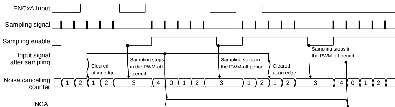
Figure 3.17 Noise Cancelling (Sampling in PWM-on Period, Noise Cancelling Timer Stops in PWM-off Period. <NCT>=4)
