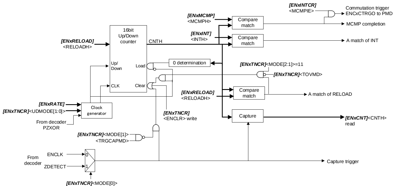
Figure 3.24 Configuration of Counter (Sensor Mode (Phase Count), and Phase Counter Mode)
