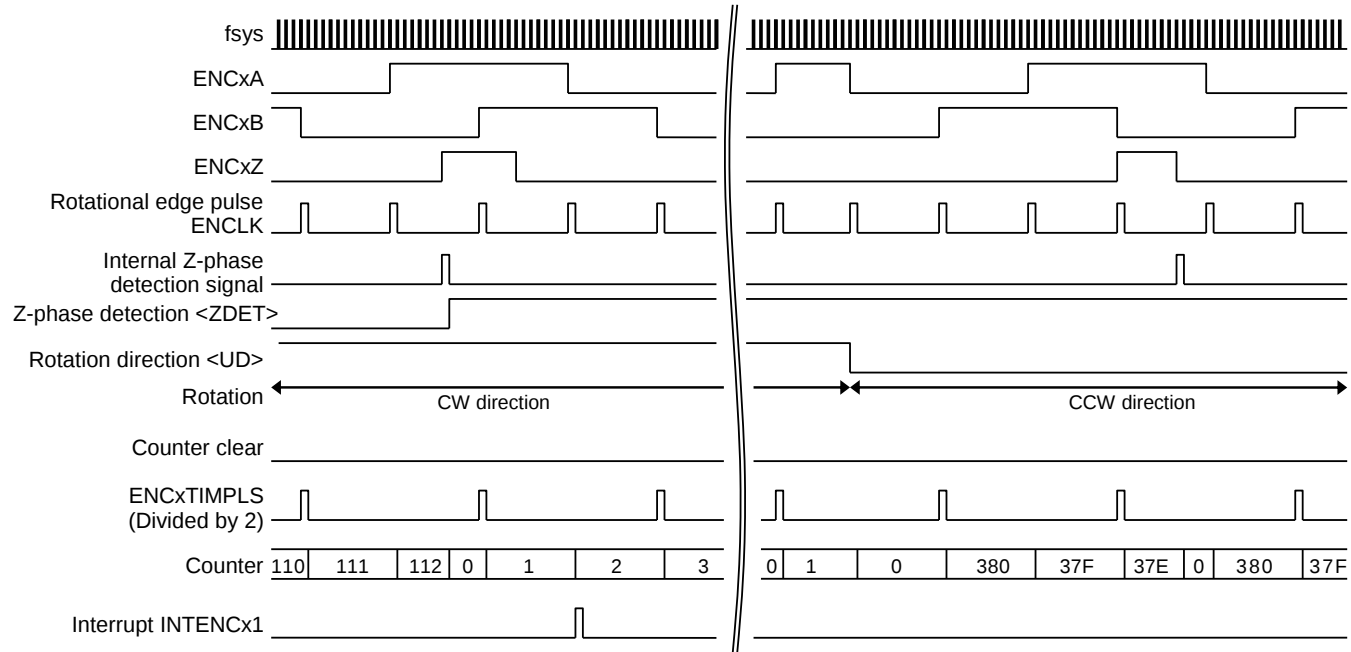
Figure 3.1 ENCxZ Input is Enabled ( [ENxTNCR]<ZEN>=1 )
