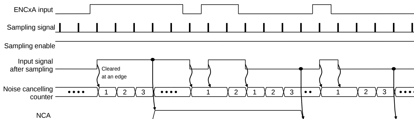
Figure 3.16 Noise Cancelling (Continuous, \langle \text{NCT} \rangle = 3 )
