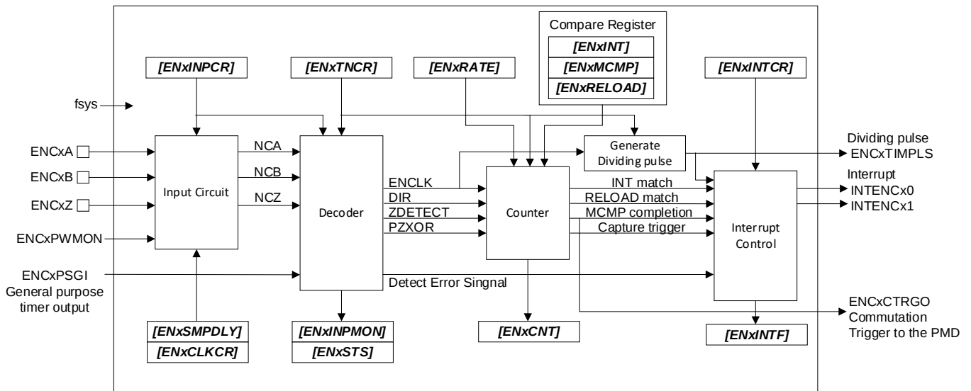
Figure 2.1 A-ENC Block Diagram
