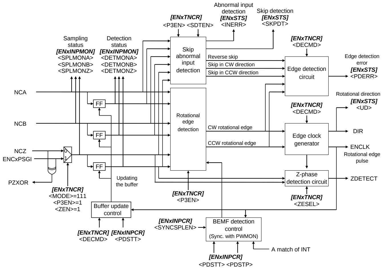
Figure 3.19 Configuration of Decoder
