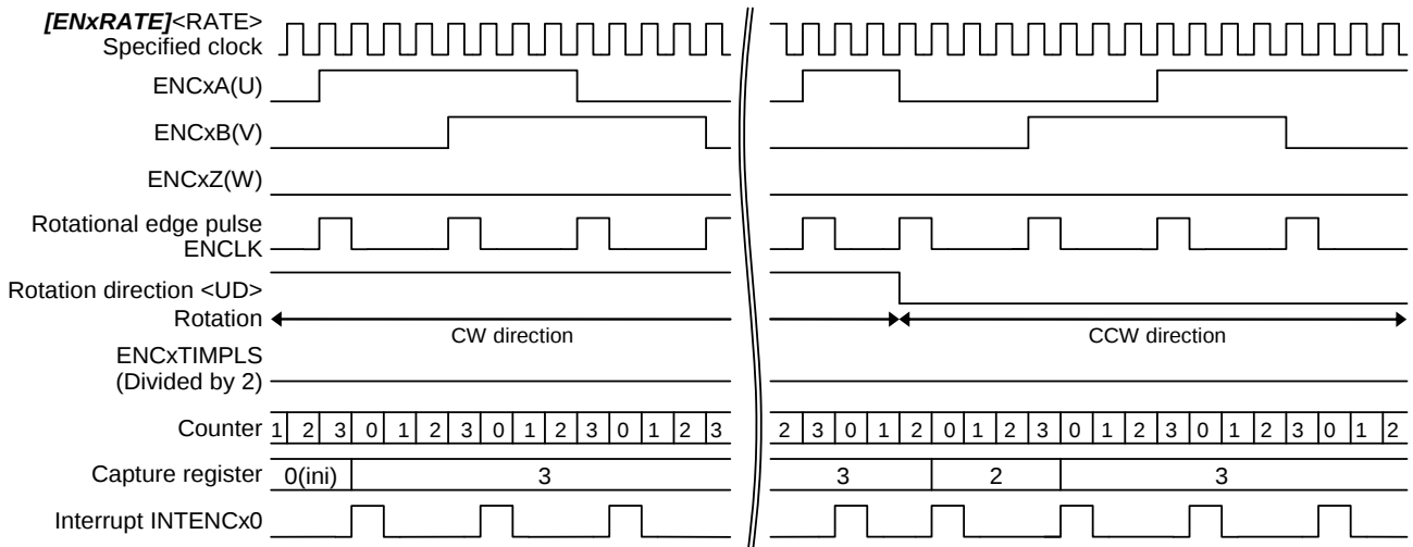
Figure 3.8 2-phase Decoding ( [ENxTNCr] \langle P3EN \rangle = 0 )
