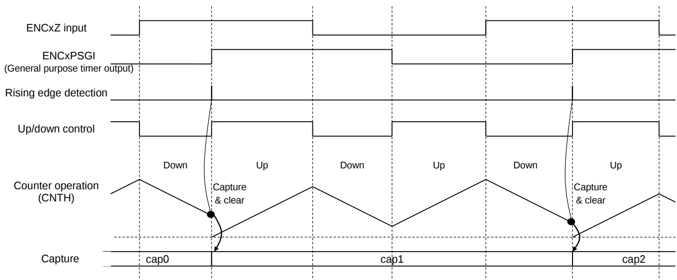
Figure 3.13 Operation in Phase Counter Mode (Phase Difference Measurement)
