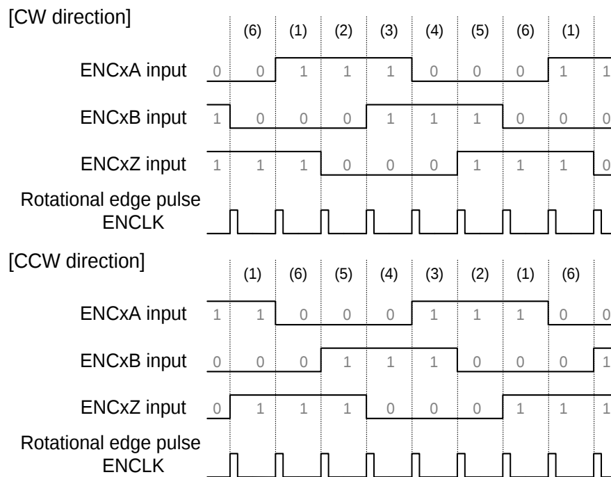
Figure 3.21 Waveforms of 3-phase Decoding
