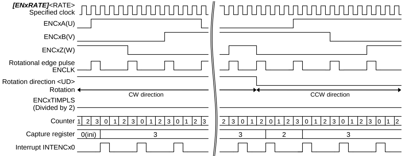
Figure 3.7 3-phase Decoding ( [ENxTNCr] \langle P3EN \rangle = 1 )
