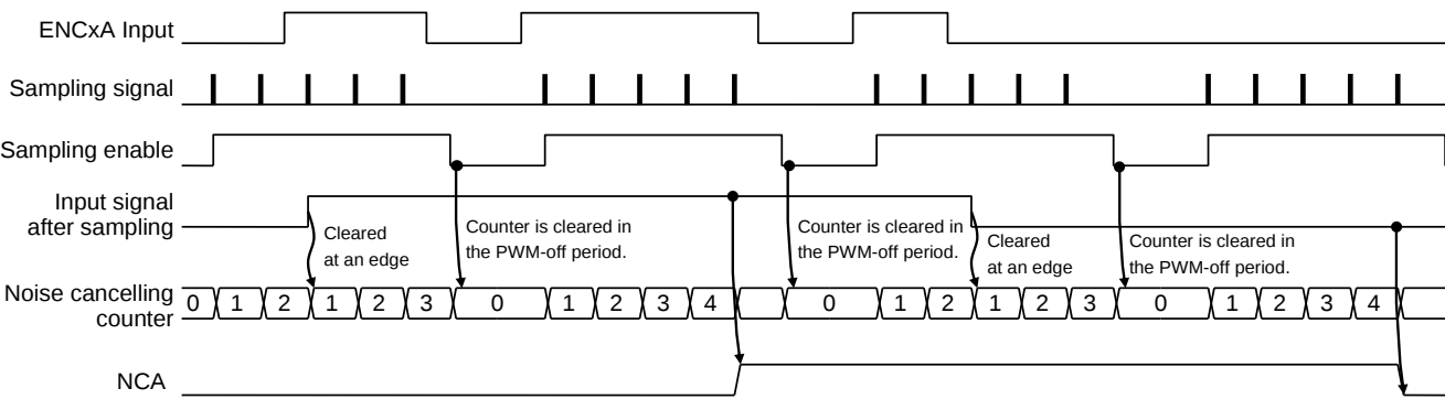
Figure 3.18 Noise Cancelling (Sampling in PWM-on Period, Noise Cancelling Timer is Cleared in PWM-off Period. <NCT>=4)
