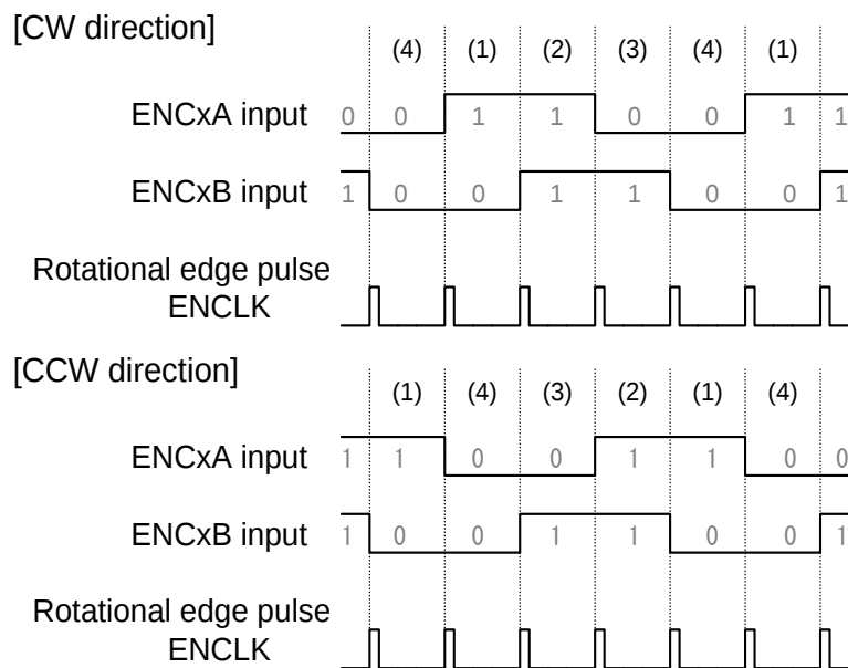
Figure 3.20 Waveforms of 2-phase Decoding
