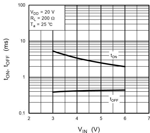
Fig. 12.7 t_{ON}, t_{OFF} - V_{IN}
