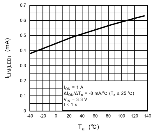
Fig. 12.12 I_{LIM(LED)} - T_a
