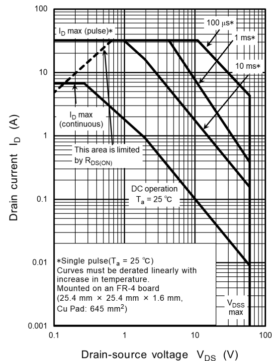
Fig. 8.9 Safe Operating Area
