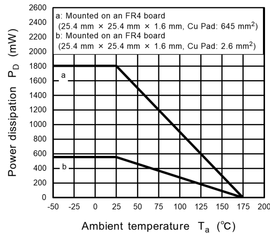
Fig. 8.11 P_D - T_a
