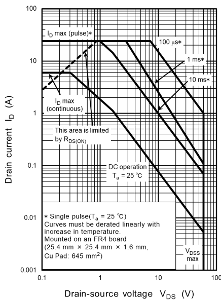
Fig. 9.10 Safe Operating Area
