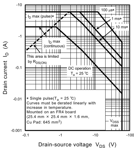
Fig. 9.10 Safe Operating Area
