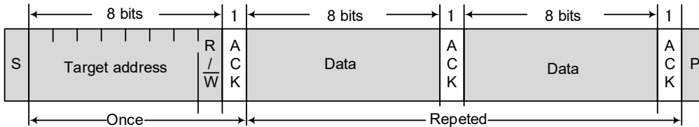
(a) 7-bit addressing format
