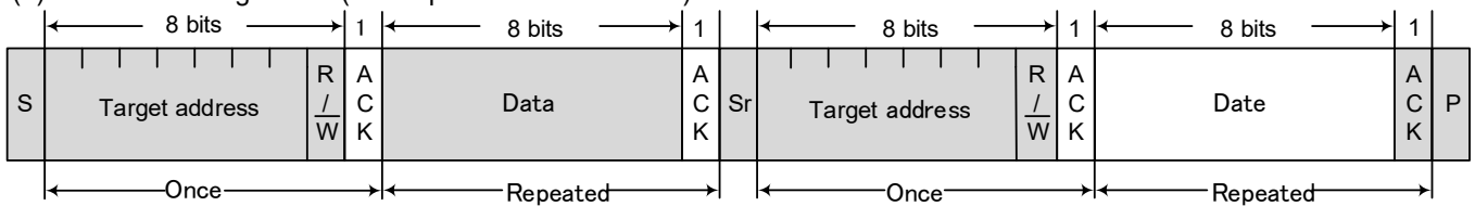
(b) 7-bit addressing format (with repeated start condition)
