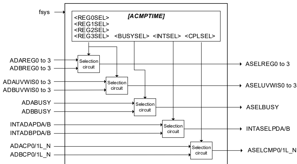
Figure 8.2 ASEL Block Diagram
