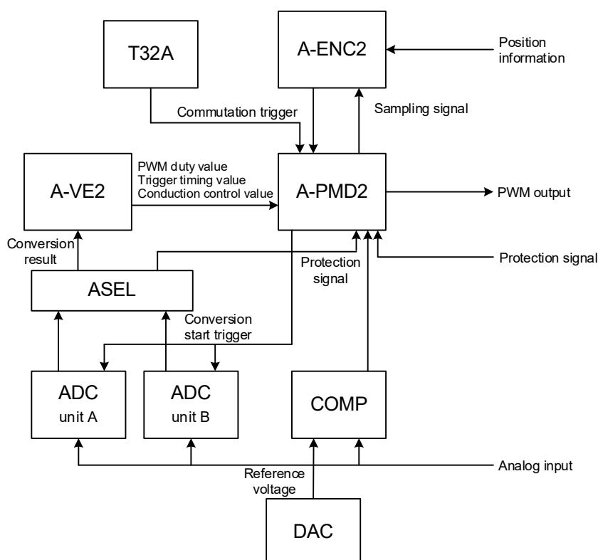
Figure 7.1 Motor Control Function Connection (Outline)
