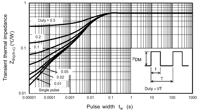
Fig. 8.13 r_{th} - t_w (Guaranteed Maximum)
