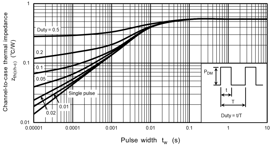
Fig. 8.15 Z_{th(ch-c)} - t_w (Guaranteed Maximum)
