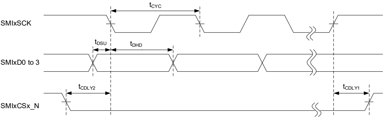
Figure 6.6 AC Timing of SMIF Read
