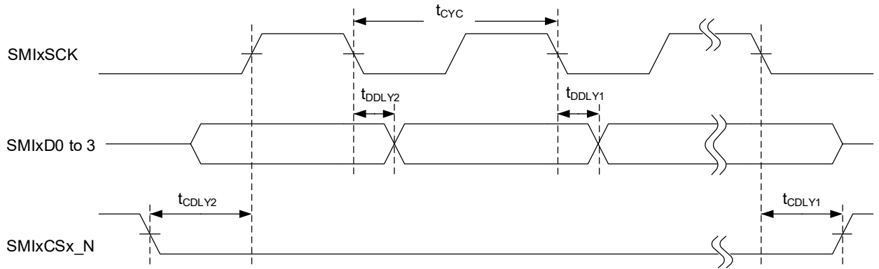
Figure 6.7 AC Timing of SMIF Write
