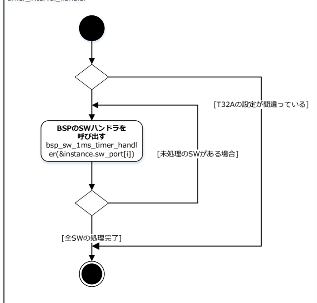
timer_interval_handler
