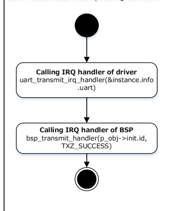
UART Transmission Interrupt calling flow chart
