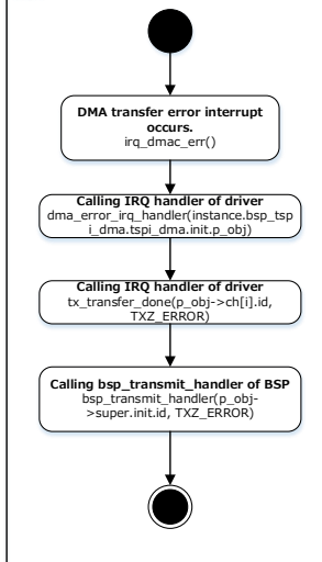
DMA Communication error Interrupt calling flow chart
