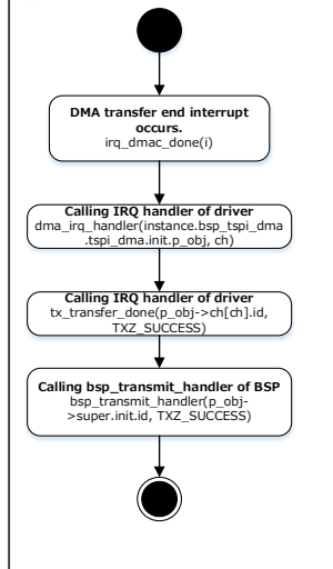
DMA Communication finished Interrupt calling flow chart
