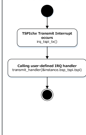
TSPI Transmit Interrupt calling flow chart
