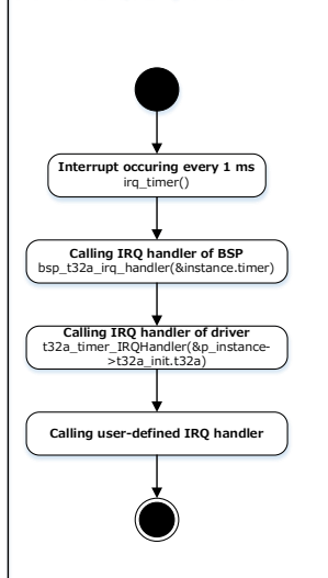
1ms Timer Interrupt calling flow chart
