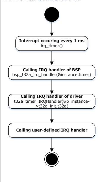
1ms Timer Interrupt calling flow chart
