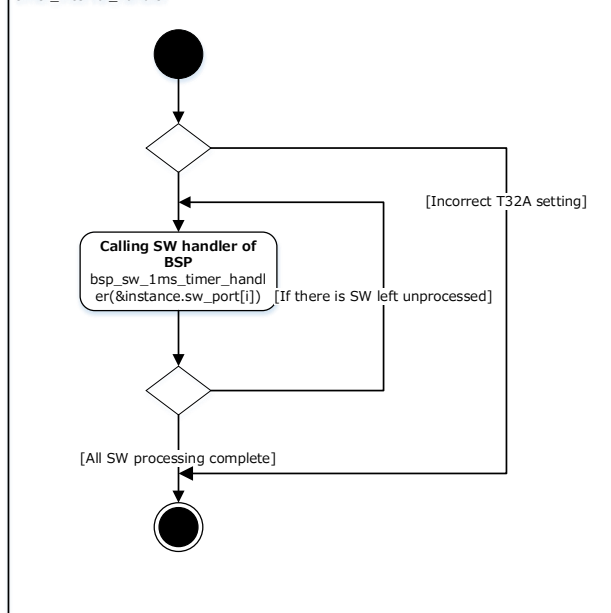
timer_interval_handler
