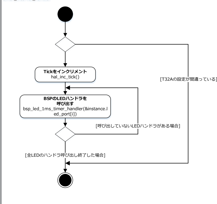
timer_interval_handler
