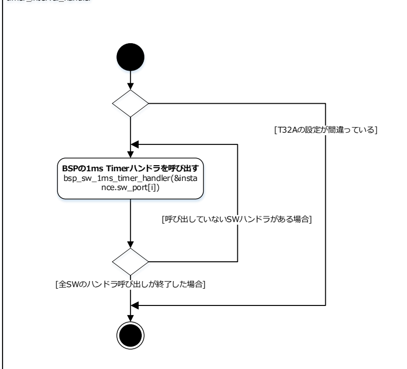
timer_interval_handler
