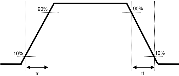
Figure 7.1 Switching characteristics
