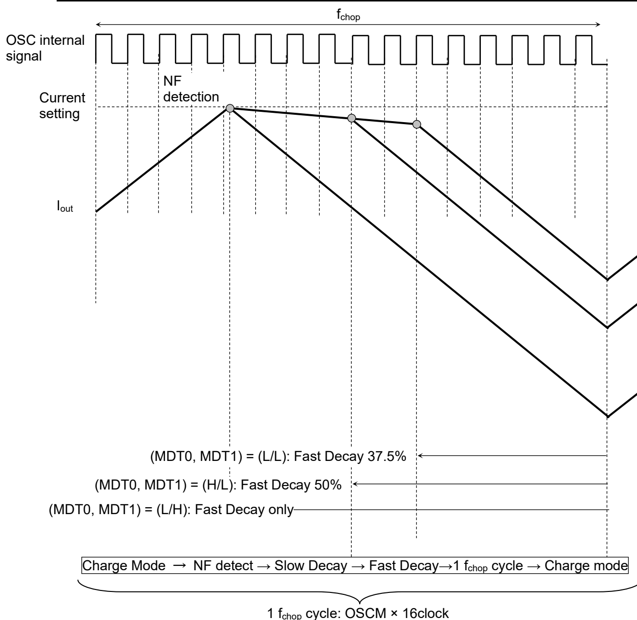
Figure 8.1 Selectable Mixed Decay function
