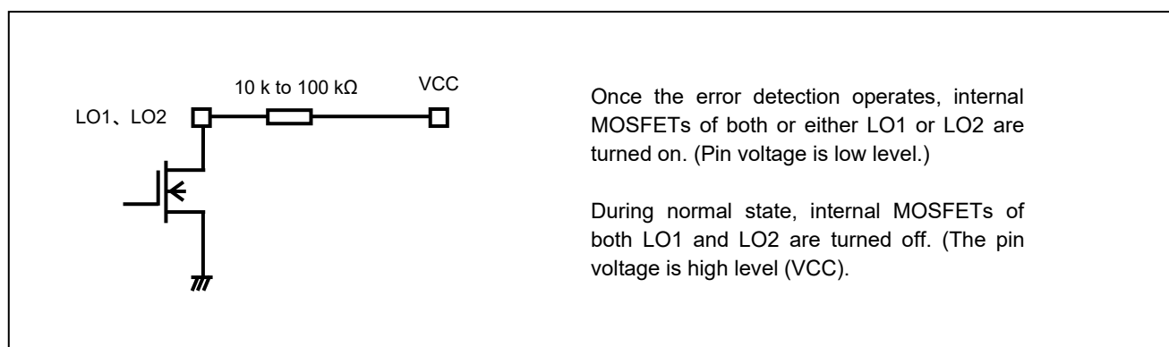
Figure 8.4 LO function Equivalent Circuit
