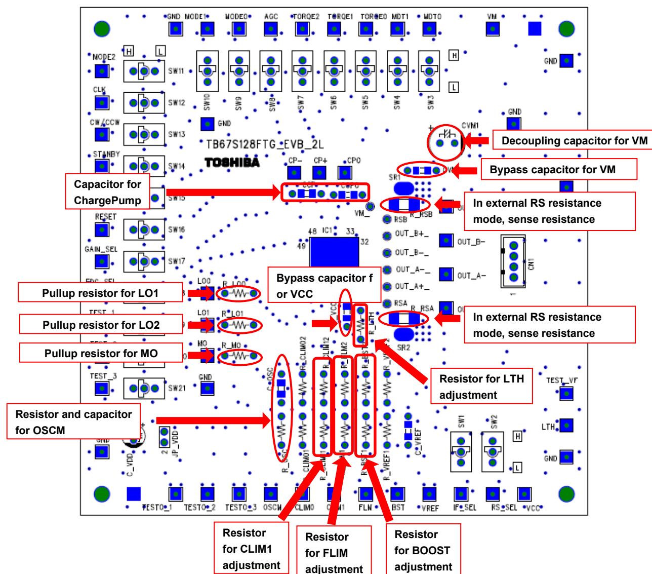
Figure 15.2 Main parts
