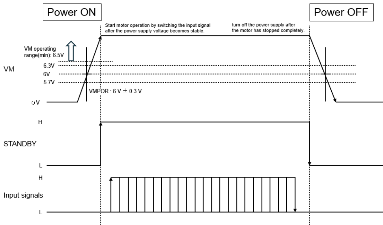
Figure 3.1 Power Supply Sequence
