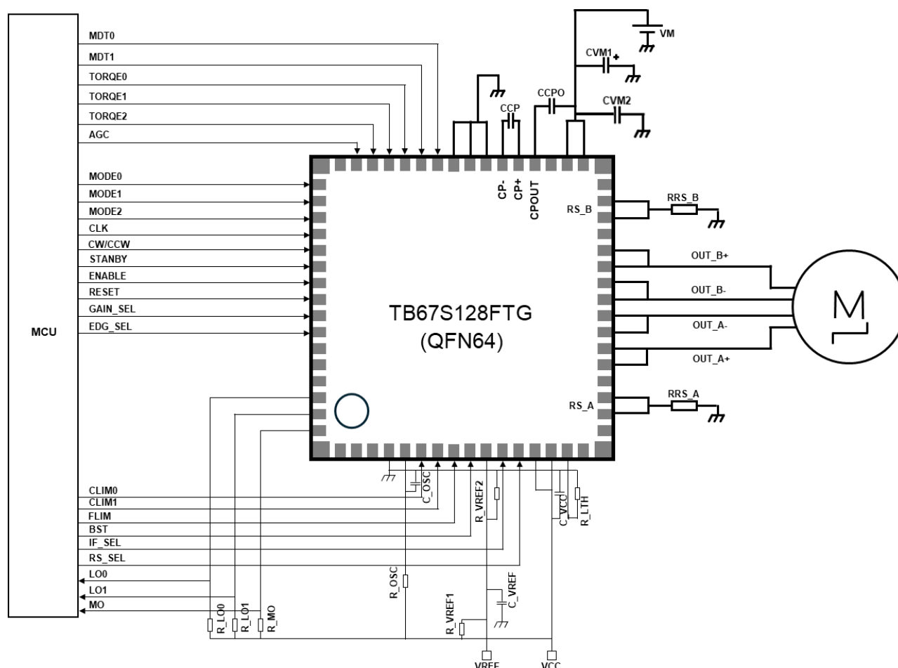
Figure 10.1 Application circuit example
