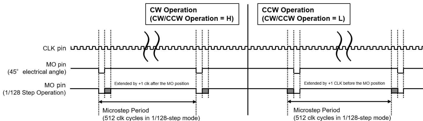
Figure 8.3 MO Pulse Width During CW/CCW Operation
