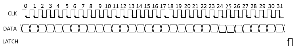
Figure 9.1 LATCH signal timing
