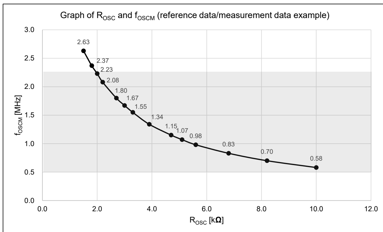
Figure 11.1 Graph of R_{OSC} and f_{OSC} (reference data/measurement data example)
