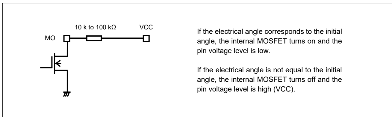
Figure 8.2 MO function Equivalent Circuit
