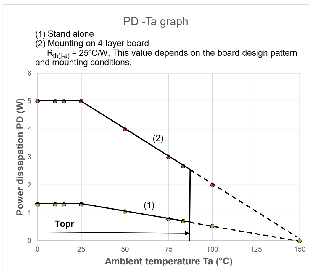
Figure 13.1 Power dissipation
