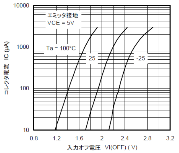
図 10.9 RN1117 I_C - V_{I(OFF)}
