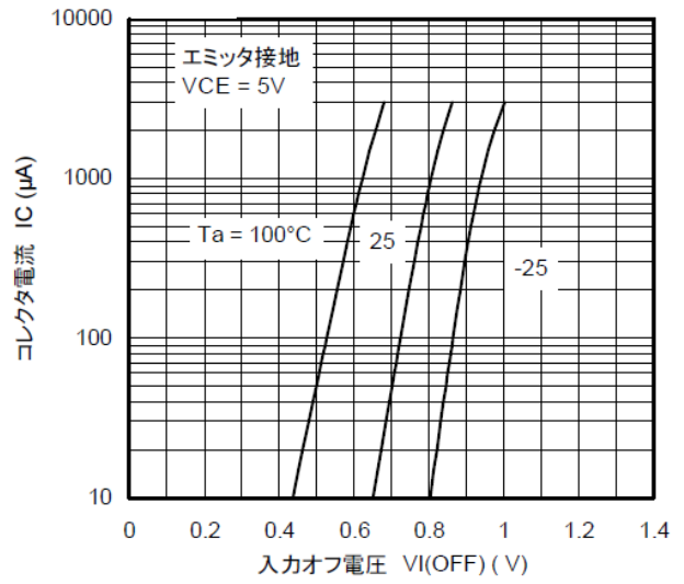
図 10.7 RN1115 I_C - V_{I(OFF)}
