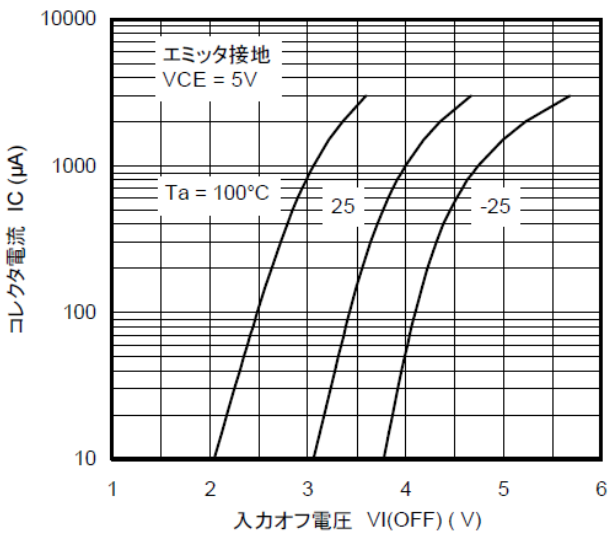
図 10.8 RN1116 I_C - V_{I(OFF)}
