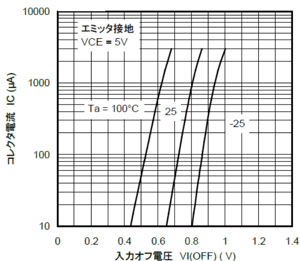
図 9.7 RN1315 I_C - V_{I(OFF)}
