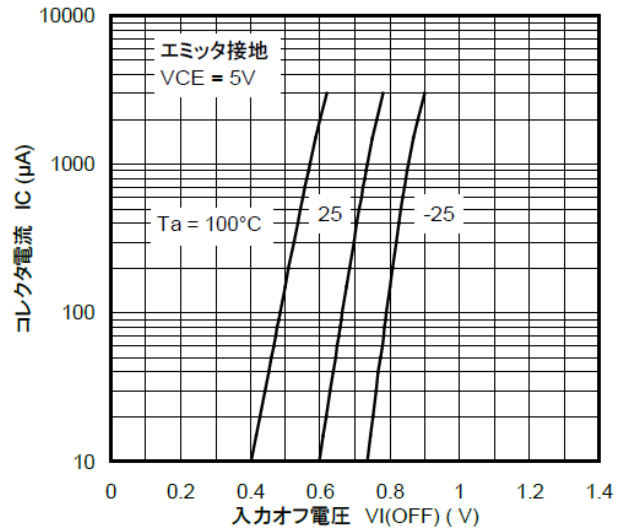
図 9.6 RN1314 I_C - V_{I(OFF)}
