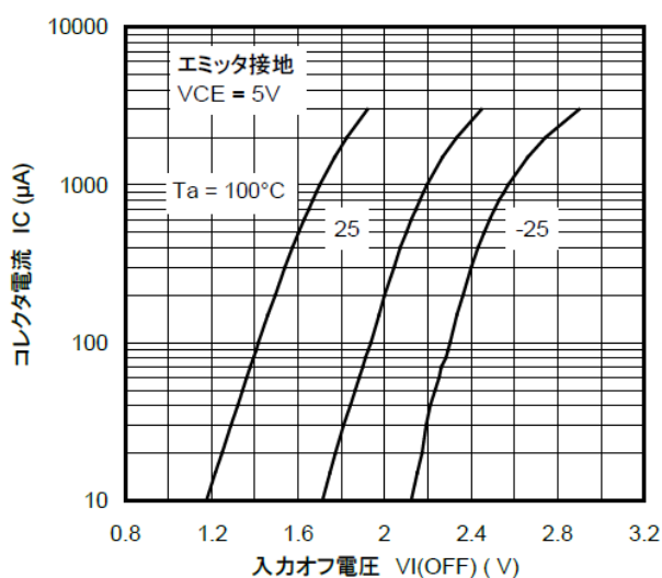
図 9.9 RN1317 I_C - V_{I(OFF)}
