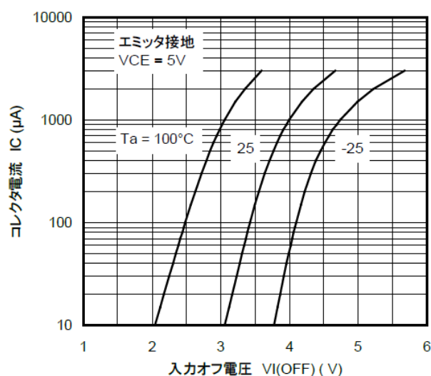
図 9.10 RN1318 I_C - V_{I(OFF)}
