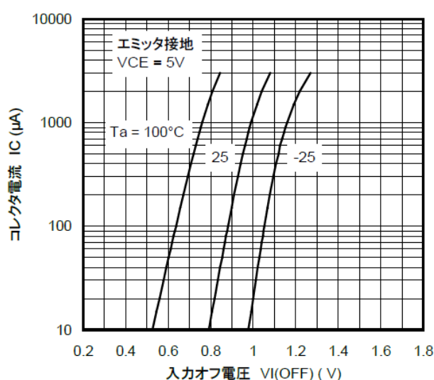
図 9.8 RN1316 I_C - V_{I(OFF)}
