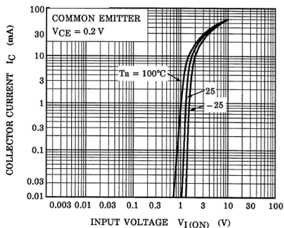
Fig. 10.1 RN1401 I_C - V_{I(ON)}
