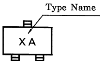
Fig. 9.1 Marking RN1401
