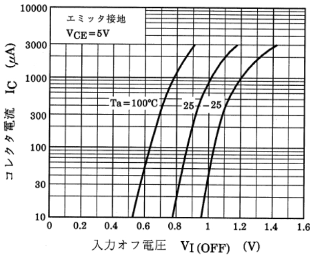
図 10.5 RN1408 I_C - V_{I(OFF)}
