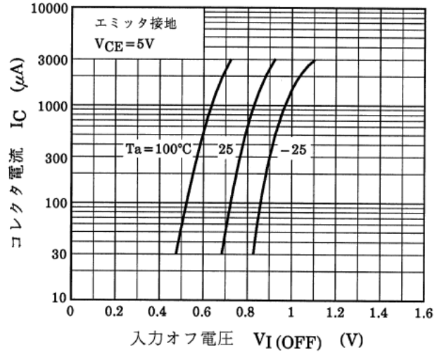
図 10.4 RN1407 I_C - V_{I(OFF)}
