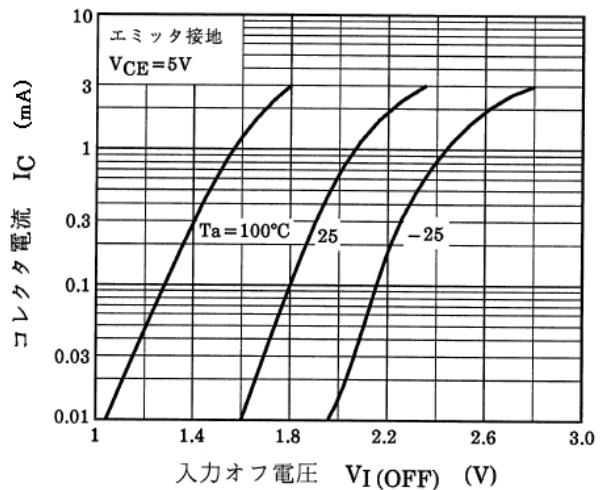
図 10.6 RN1409 I_C - V_{I(OFF)}
