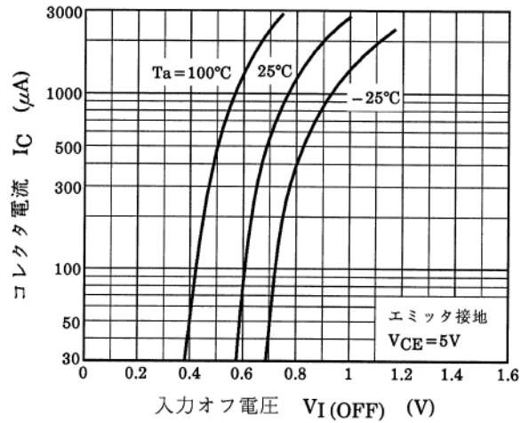
図 9.4 RN1413 I_C - V_{I(OFF)}
