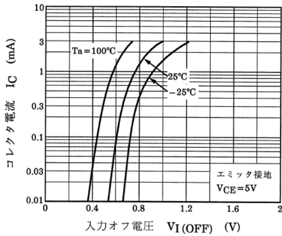
図 9.3 RN1412 I_C - V_{I(OFF)}
