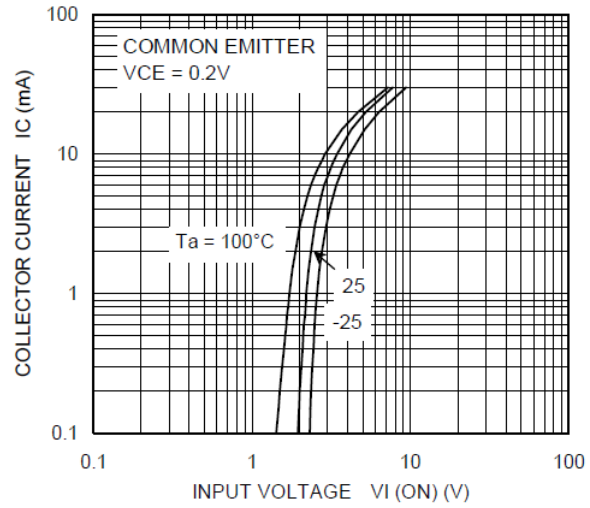
Fig. 10.4 RN1417 I_C - V_{I(ON)}
