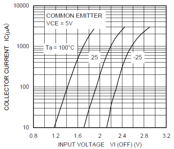
Fig. 10.9 RN1417 I_C - V_I (OFF)
