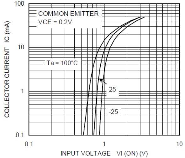
Fig. 10.2 RN1415 I_C - V_{I(ON)}
