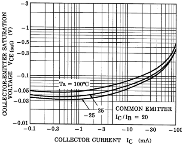
Fig. 9.8 RN2111 V_{CE(sat)}-I_C
