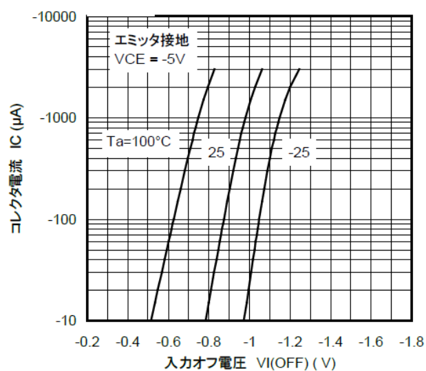
図 10.8 RN2116 I_C - V_{I(OFF)}
