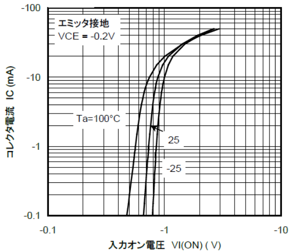
図 10.1 RN2114 I_C - V_{I(ON)}
