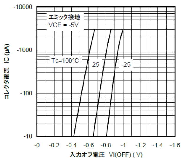
図 10.7 RN2115 I_C - V_{I(OFF)}
