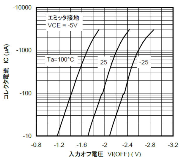
図 10.9 RN2117 I_C - V_{I(OFF)}
