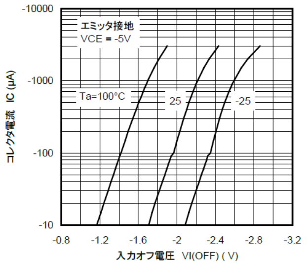
図 10.9 RN2117 I_C - V_{I(OFF)}
