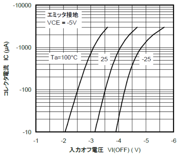
図 10.8 RN2116 I_C - V_{I(OFF)}
