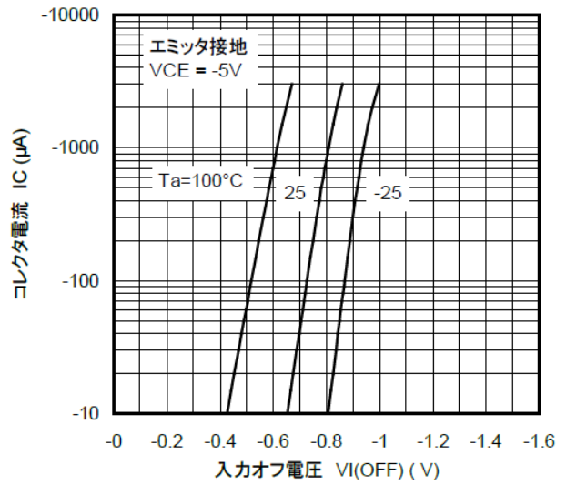
図 10.7 RN2115 I_C - V_{I(OFF)}
