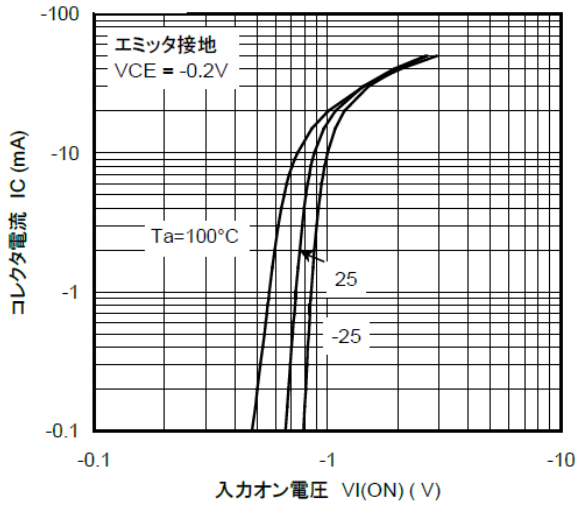
図 10.1 RN2114 I_C - V_{I(ON)}
