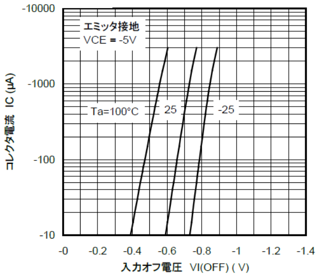
図 10.6 RN2114 I_C - V_{I(OFF)}
