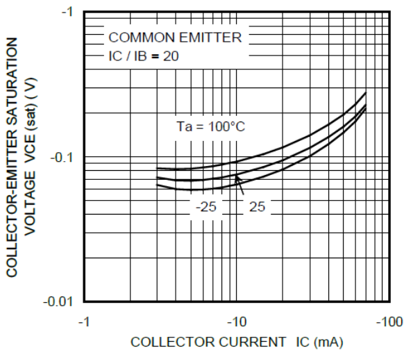
Fig. 10.20 RN2118 V_{CE(sat)}-I_C
