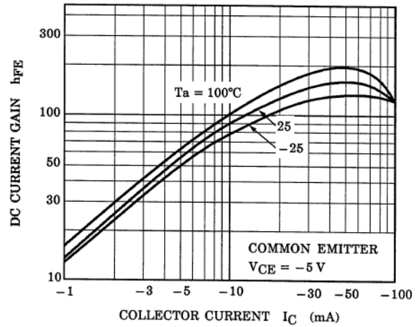
Fig. 10.14 RN2402 h_{FE-IC}
