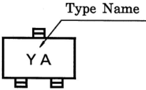
Fig. 9.1 Marking RN2401
