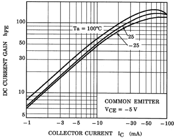
Fig. 10.13 RN2401 h_{FE-IC}
