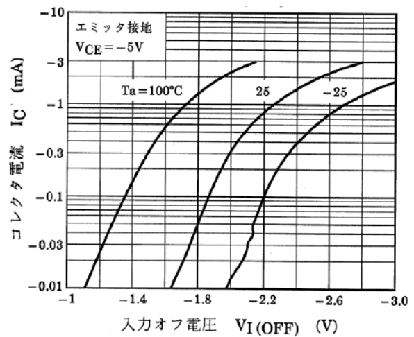
図 10.6 RN2409 I_C - V_{I(OFF)}
