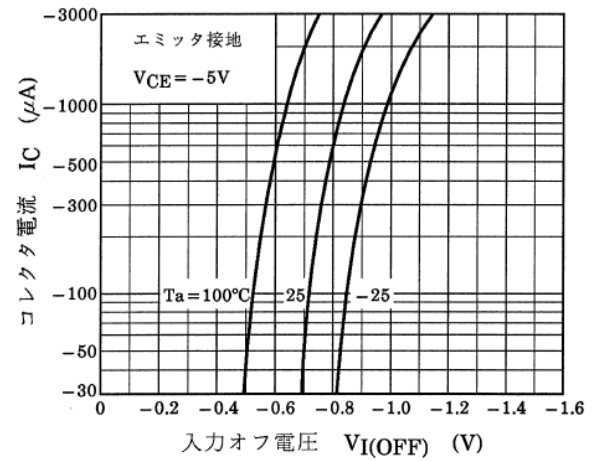
図 10.4 RN2407 I_C - V_{I(OFF)}
