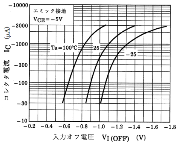
図 10.5 RN2408 I_C - V_{I(OFF)}
