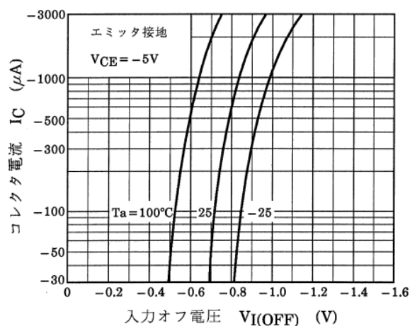
図 7.2 RN2607 I_C - V_{I(OFF)}
