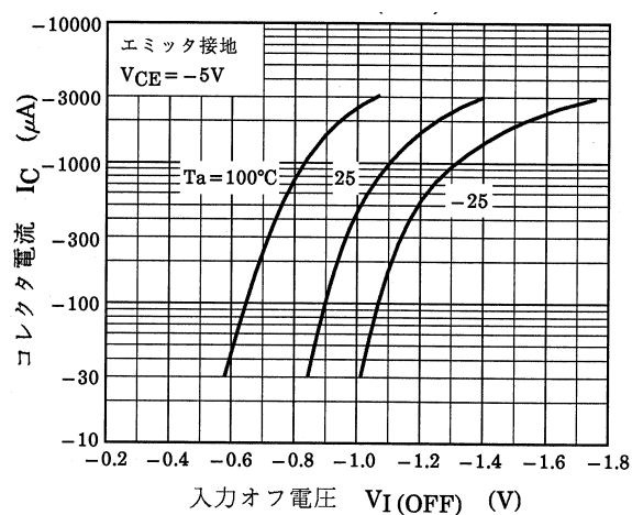
図 7.4 RN2608 I_C - V_{I(OFF)}
