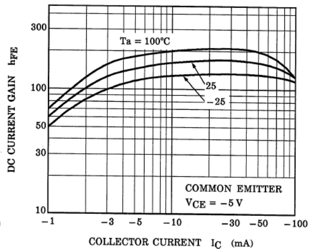
Fig. 10.18 RN2906 h_{FE-IC}
