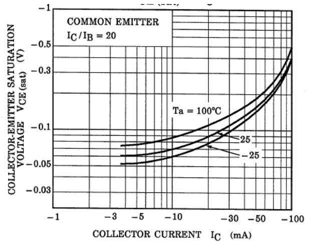
Fig. 10.20 RN2902 V_{CE(sat)}-I_C
