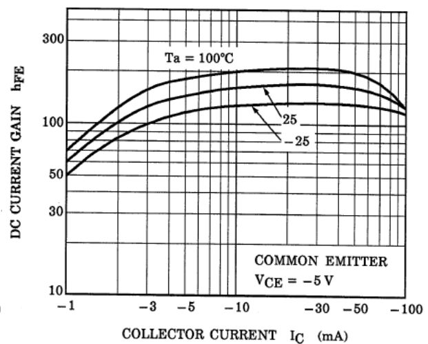
Fig. 10.18 RN2906 h_{FE-IC}
