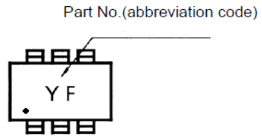
Fig. 9.6 Marking RN2906
