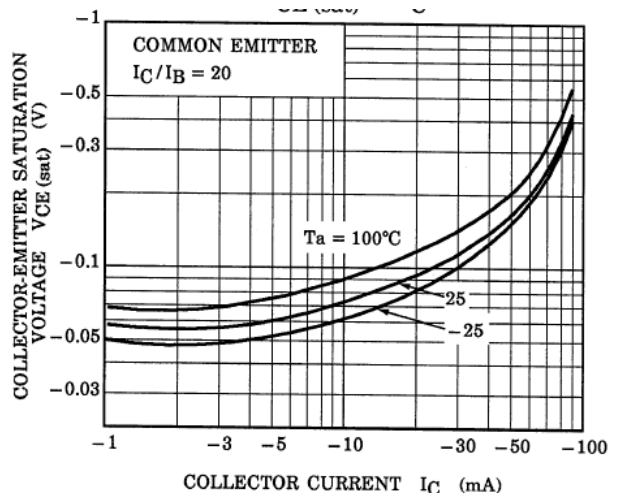
Fig. 10.24 RN1206 V_{CE(sat)}-I_C
