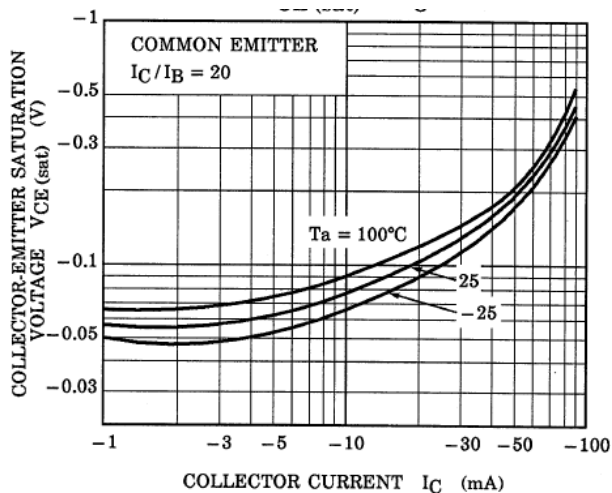
Fig. 10.23 RN2905 V_{CE(sat)}-I_C
