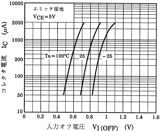
図 12.5 Q2 I_C - V_{I(OFF)}
