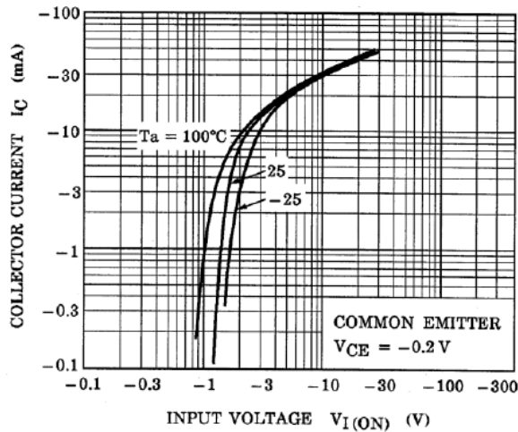
Fig. 10.3 RN2303 I_C - V_{I(ON)}
