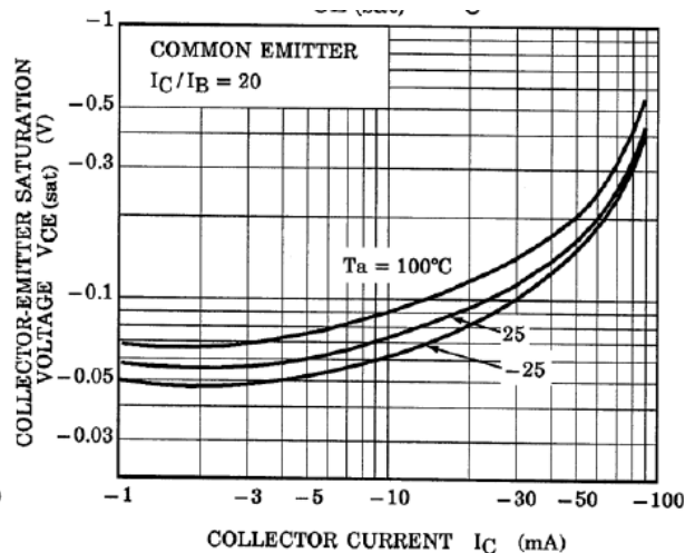
Fig. 10.24 RN2306 V_{CE(sat)}-I_C
