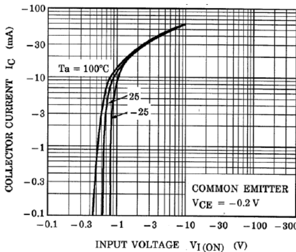
Fig. 10.5 RN2305 I_C - V_{I(ON)}
