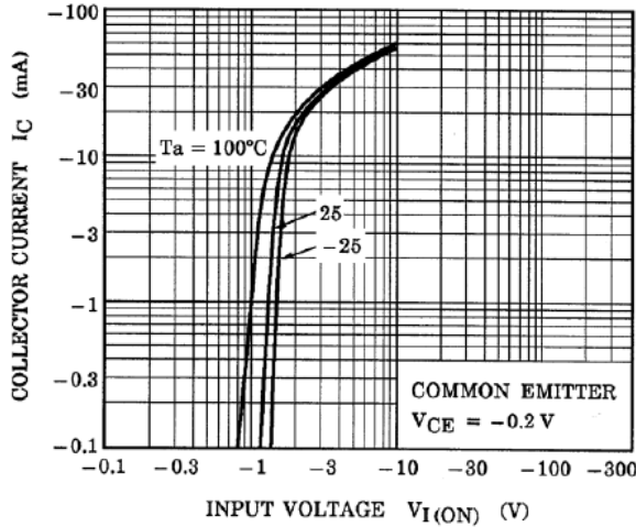
Fig. 10.1 RN2301 I_C - V_{I(ON)}
