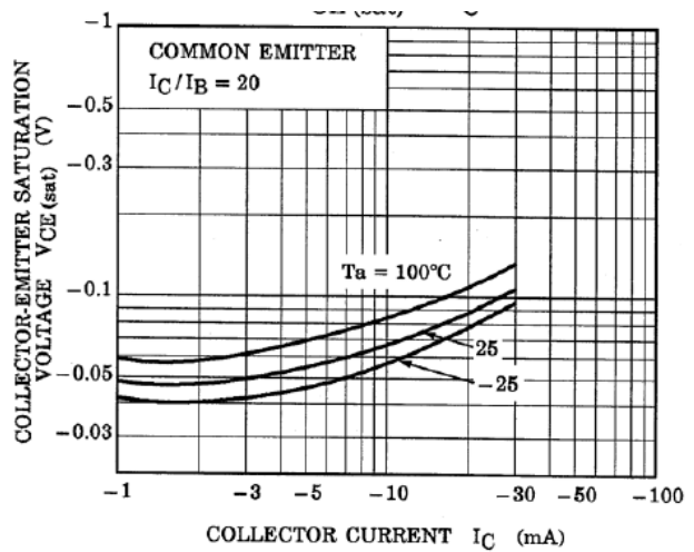
Fig. 10.22 RN2304 V_{CE(sat)}-I_C
