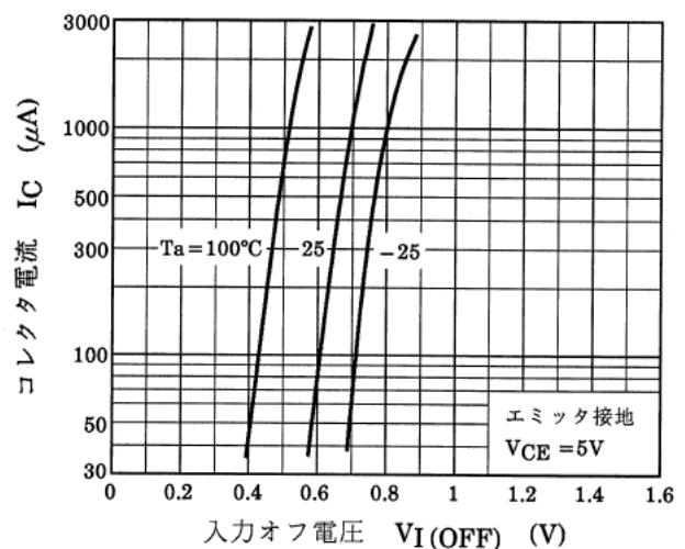
図 9.4 RN1911FE I_C - V_{I(OFF)}
