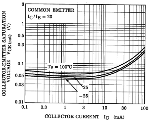
Fig. 9.8 RN1911FE V_{CE(sat)} - I_C
