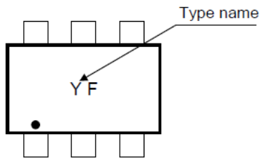
Fig. 9.6 Marking RN2906FE
