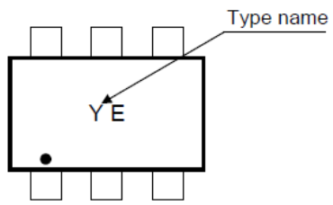
Fig. 9.5 Marking RN2905FE
