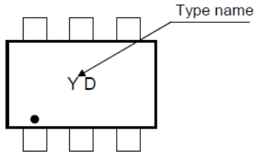
Fig. 9.4 Marking RN2904FE
