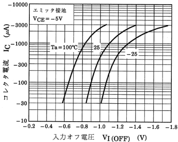
図 10.5 RN2908FE I_C - V_{I(OFF)}
