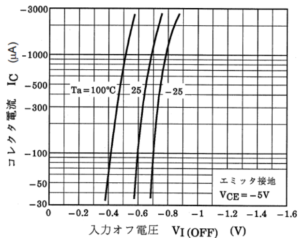
図 9.4 RN2911FE I_C - V_{I(OFF)}
