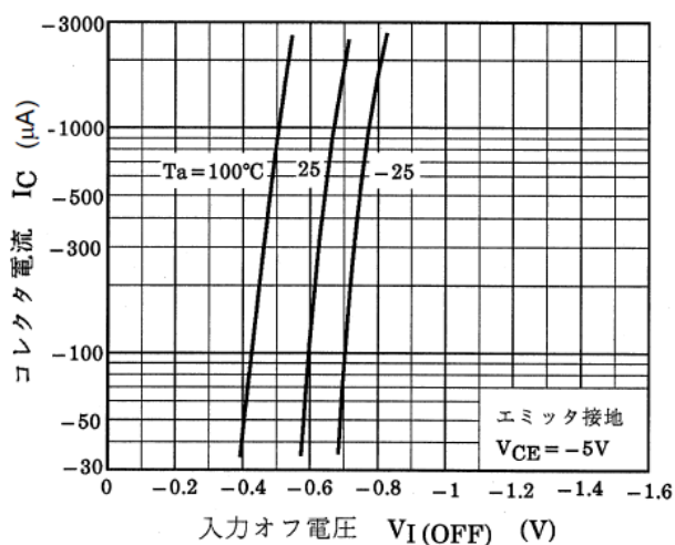
図 9.3 RN2910FE I_C - V_{I(OFF)}
