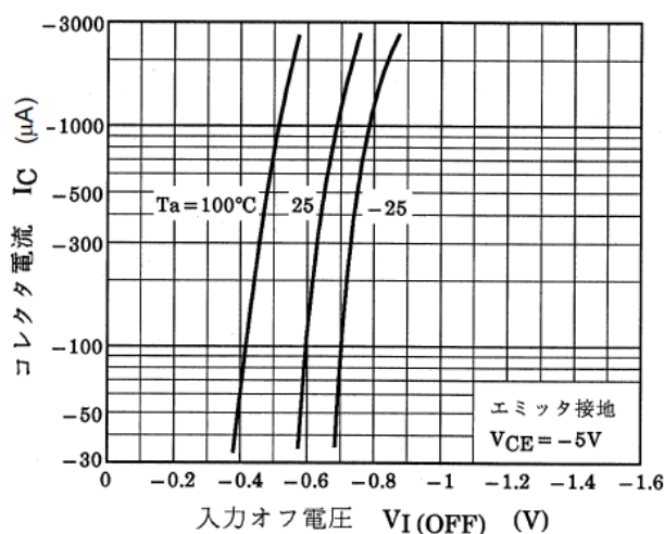
図 9.4 RN2911FE I_C - V_{I(OFF)}
