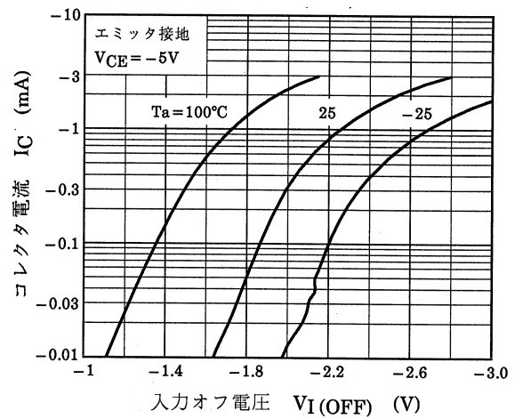
図 7.6 RN2709JE I_C - V_{I(OFF)}
