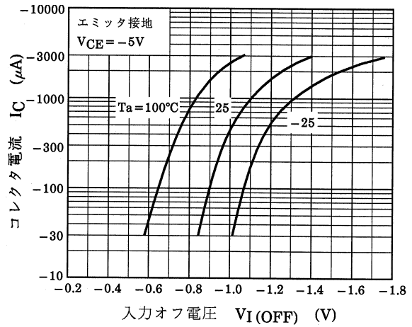
図 7.4 RN2708JE I_C - V_{I(OFF)}
