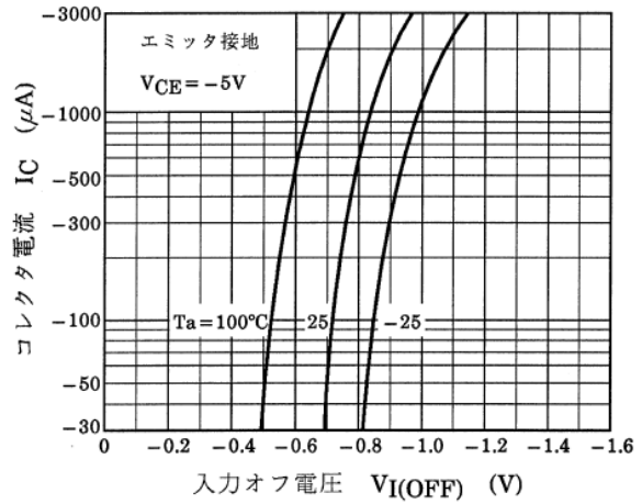
図 7.2 RN2707JE I_C - V_{I(OFF)}
