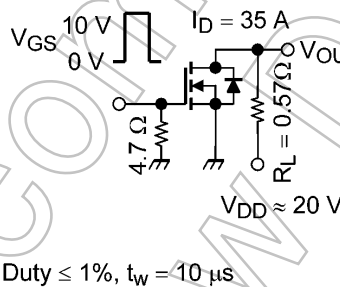
Fig. 6.2.1 Switching Time Test Circuit
