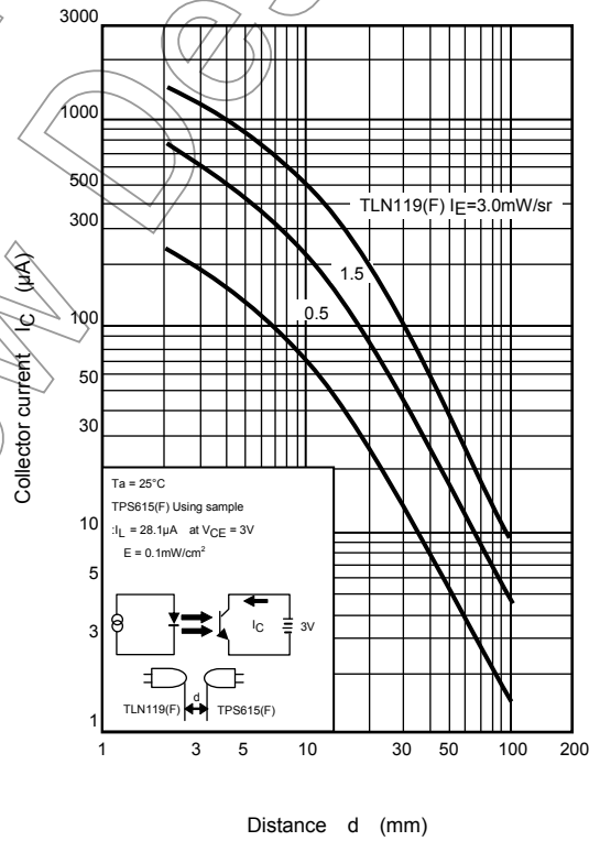
Coupling Characteristics With TLN119(F)
