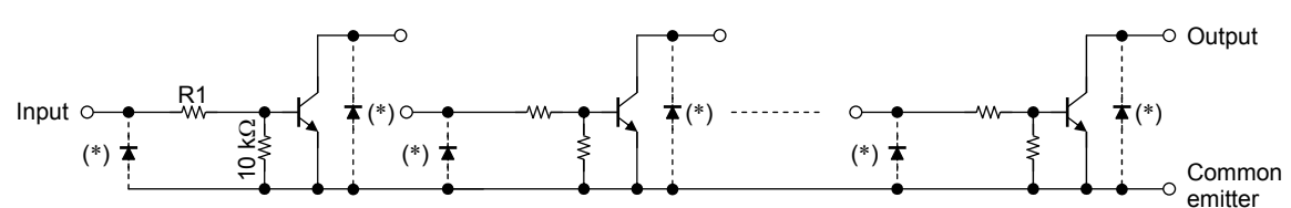
TD62503FNG
